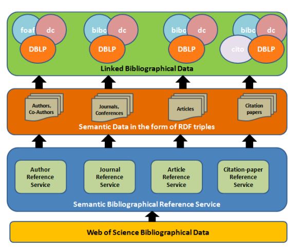
Fig. 1. Semantic Bibliographical Reference Service Infrastructure
